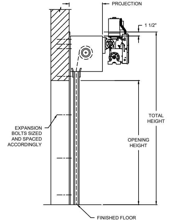
SECTION B-B
