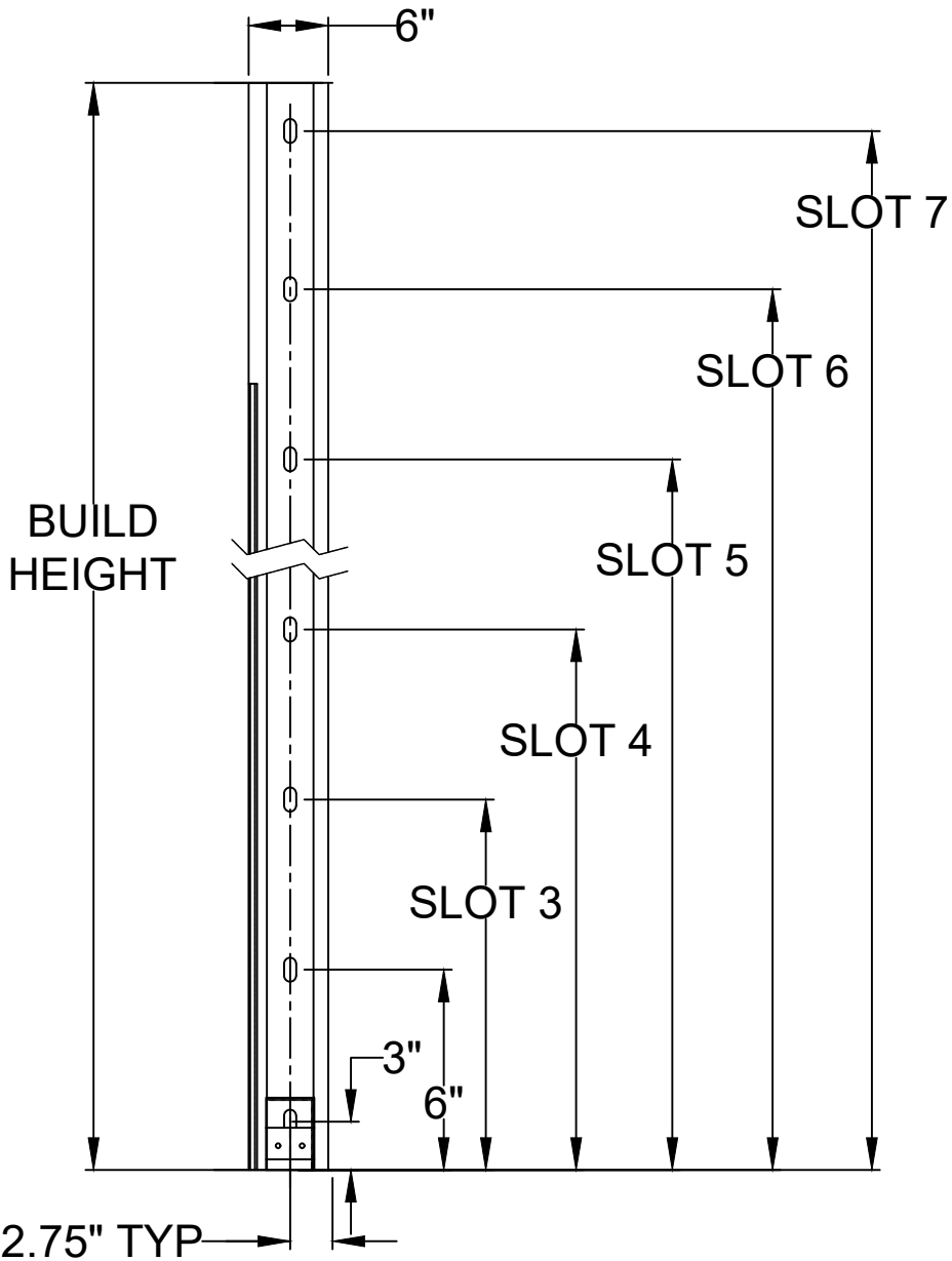
JAMB DETAIL SHOWING 7 SLOTS
